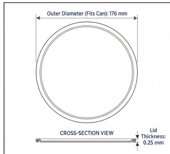
TOP VIEW & CROSS-SECTION
